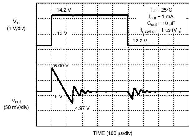
Figure 16. Line Transients
